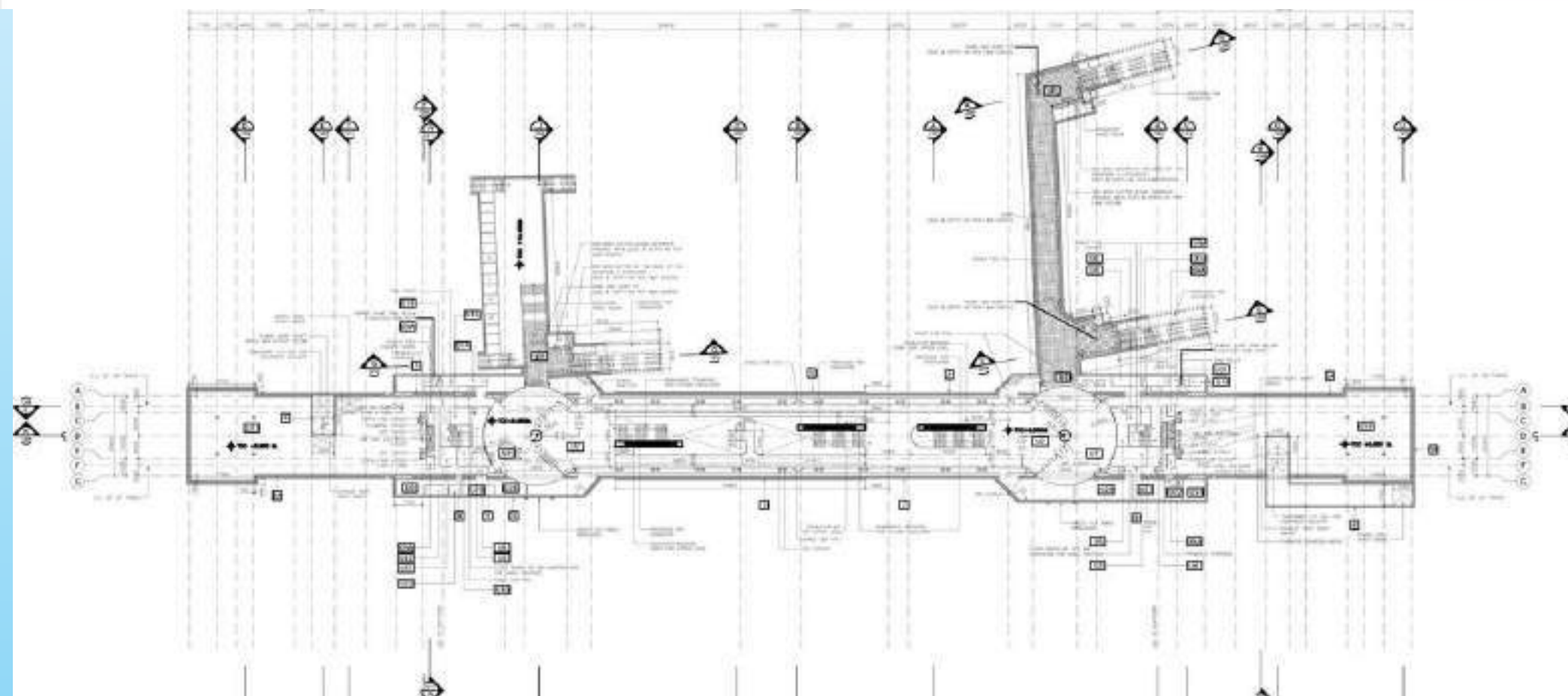
DMRC Section Shaft
